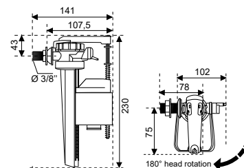
lateral, brass 3/8" with 1/2" adapter
