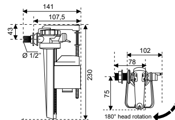
lateral, brass 1/2"
